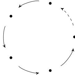
Figure 11: Cyclic quiver \tilde{A}_{n-1}
