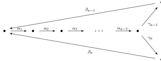
Figure 13: The quiver Q
